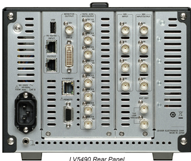
LV5490 Rear Panel
